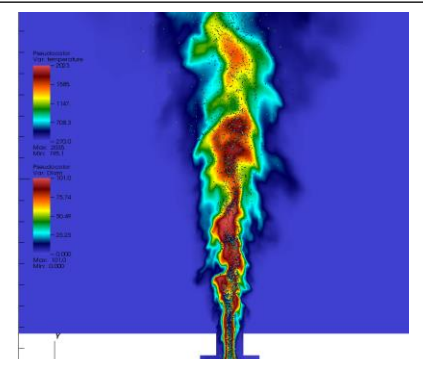
Instantaneous temperature field with droplets
